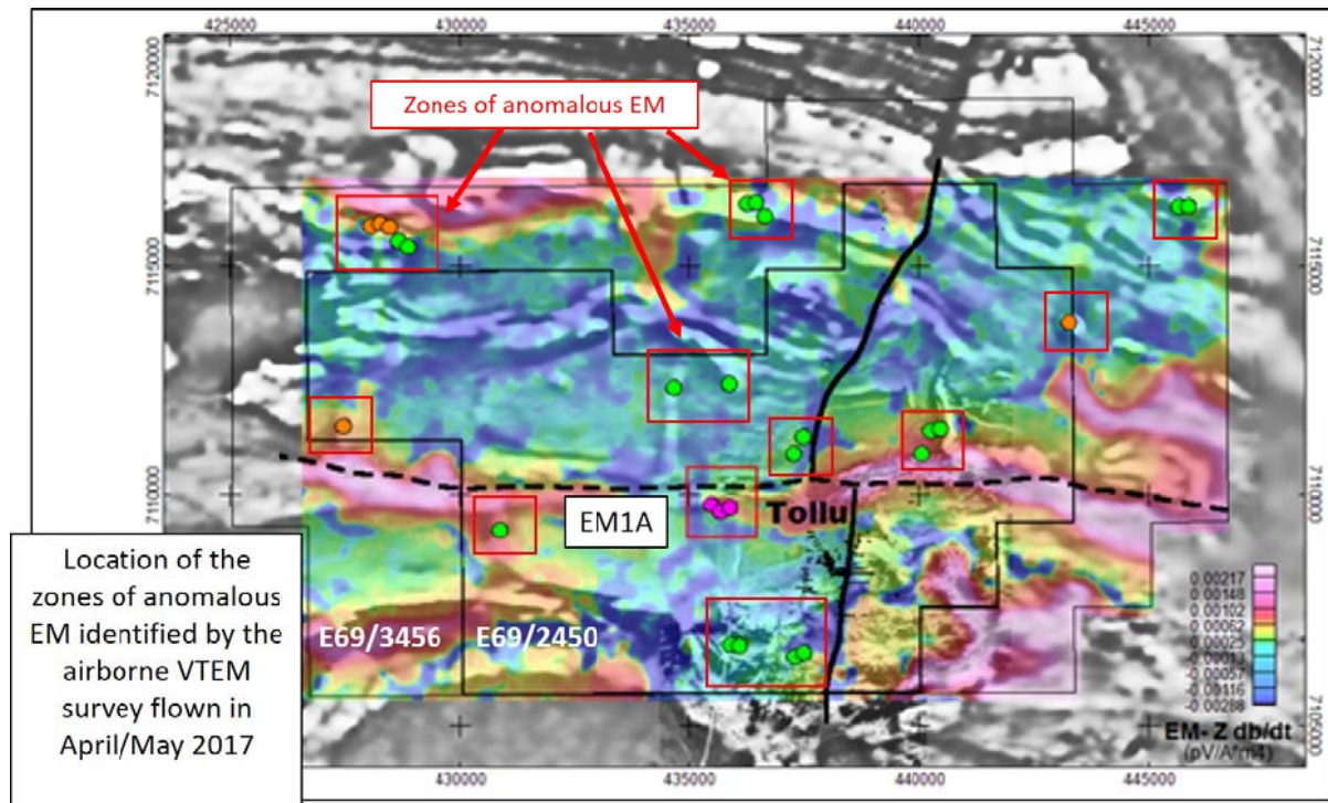
Figure 2 -- Location of EM anomalies in relation to the Tollu structural corridor. Tenement E69/2450 airborne magnetic image (grey) with late time Z component channel 48 (10.667 msec after turn off) as the colour image.
