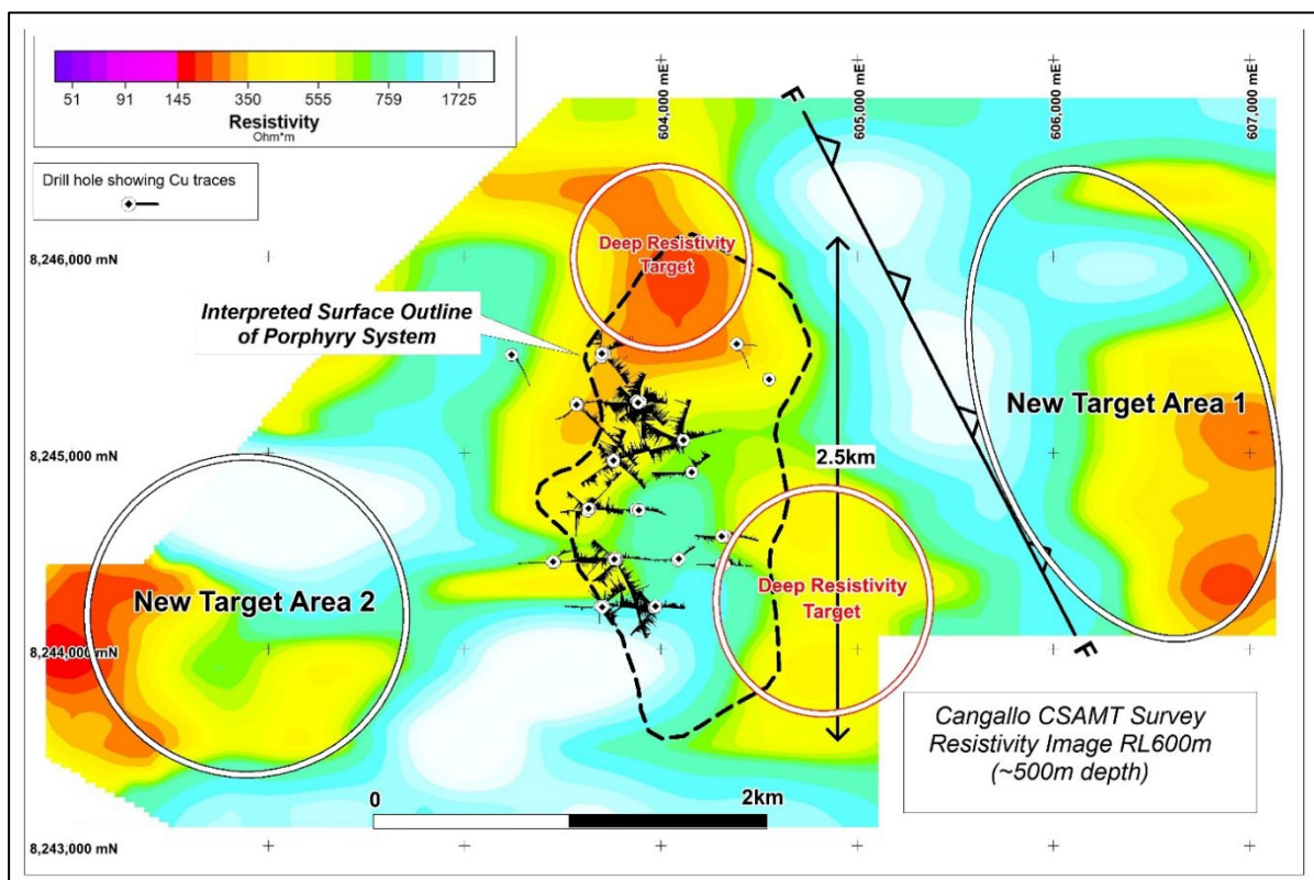
Figure 2: Cangallo CSAMT Resistivity Image (plan view) at ~500m depth showing the interpreted outline of the mineralised porphyry and additional target areas for testing.
