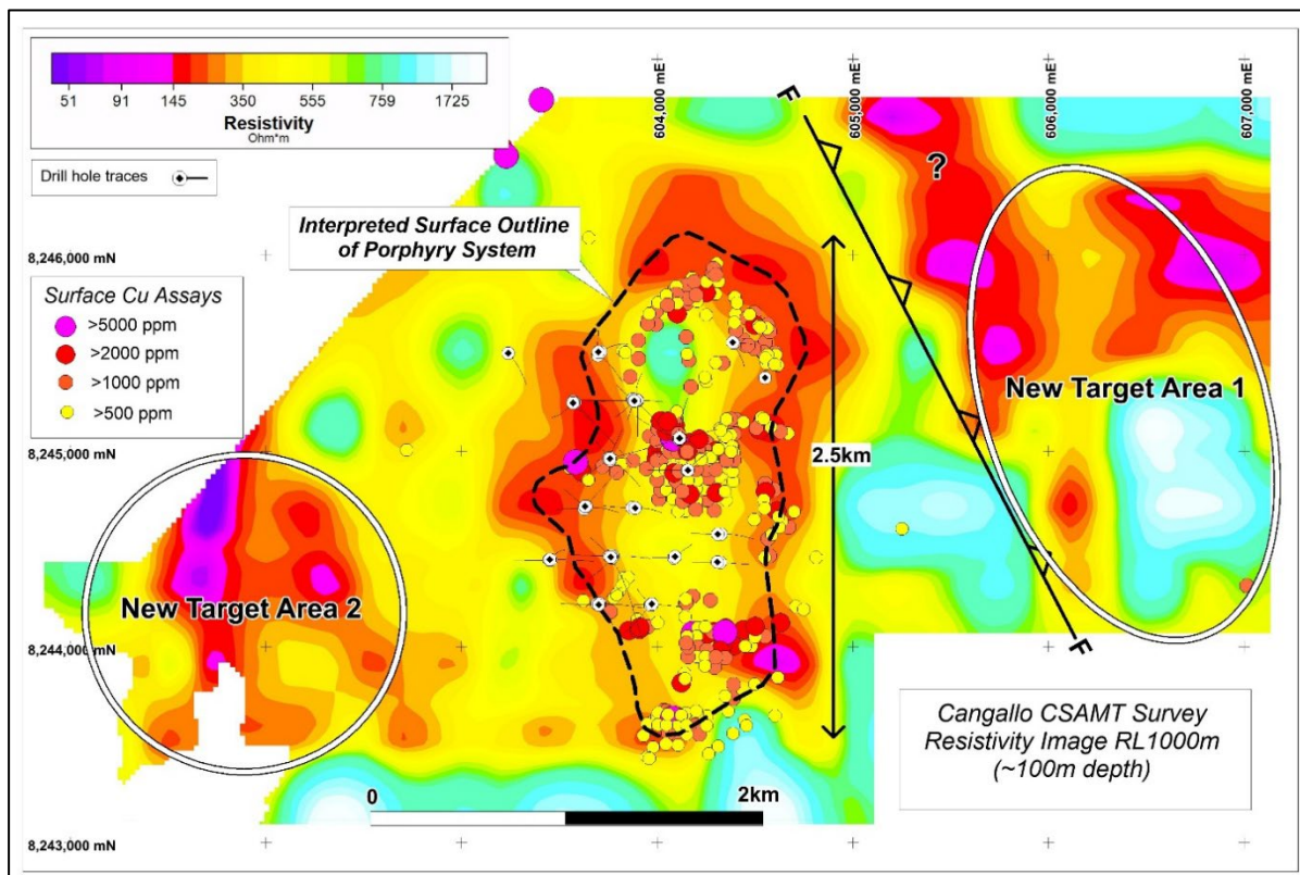
Figure 1: Cangallo CSAMT Resistivity Image (plan view) at ~100m depth showing the interpreted outline of the mineralised porphyry and additional high-priority target areas for testing (surface rock-chip assays first reported in ASX releases – 30 March and 09 November 2023)
